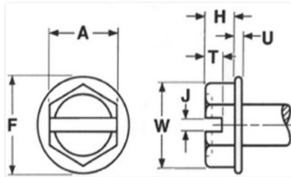
Slotted Hex Washer Head
